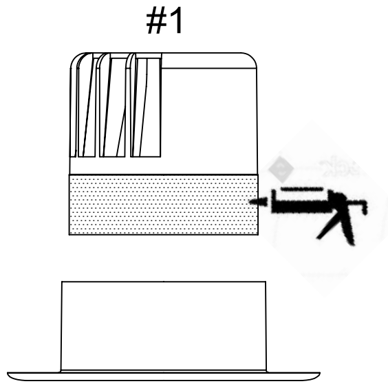
Figure 3: floor vent installation guide
